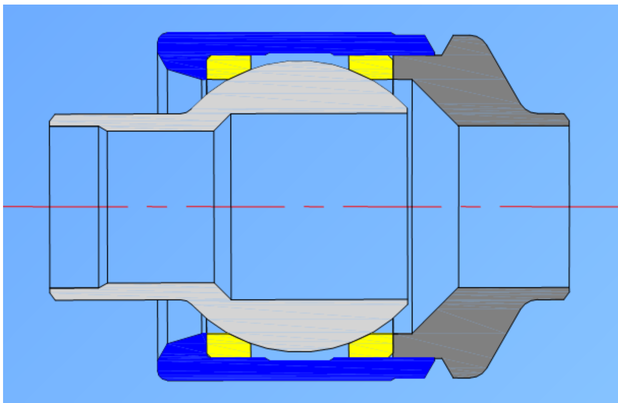
Figure 4. Restrained expansion joint.
